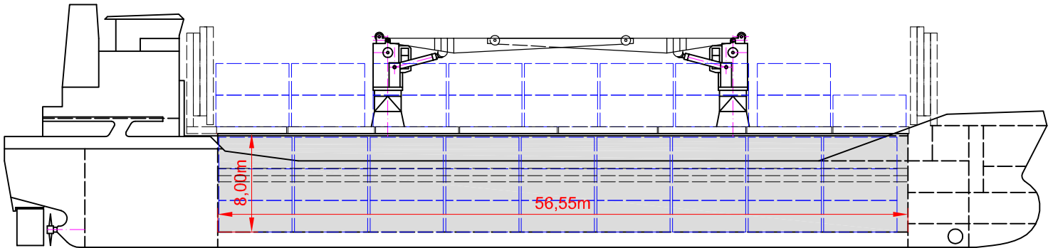
MAIN DECK
